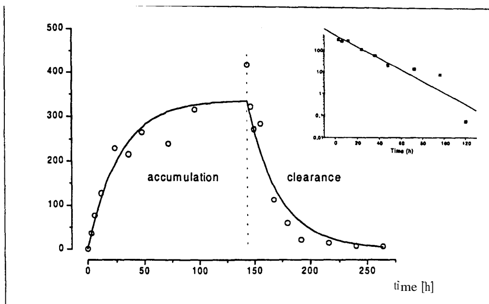
Figure 3: Kinetics of accumulation and clearance of Triclosan in zebra fish at pH 7. Triclosan concentration in water: 50 p.g/l. Top right: clearance displayed in logarithmic scale
