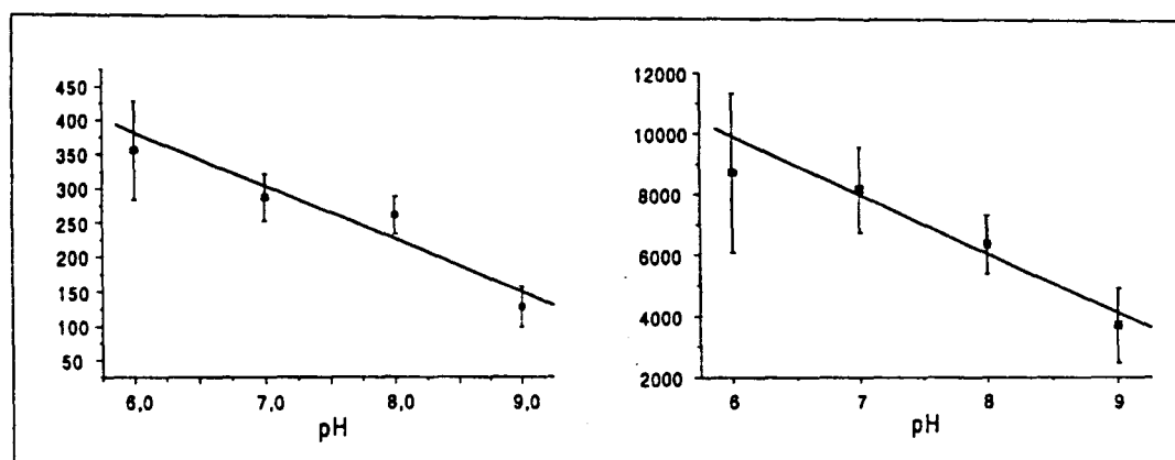
Figure 4: Uptake rate (left) and bioconcentration factor (right) versus pH of water for Triclosan
